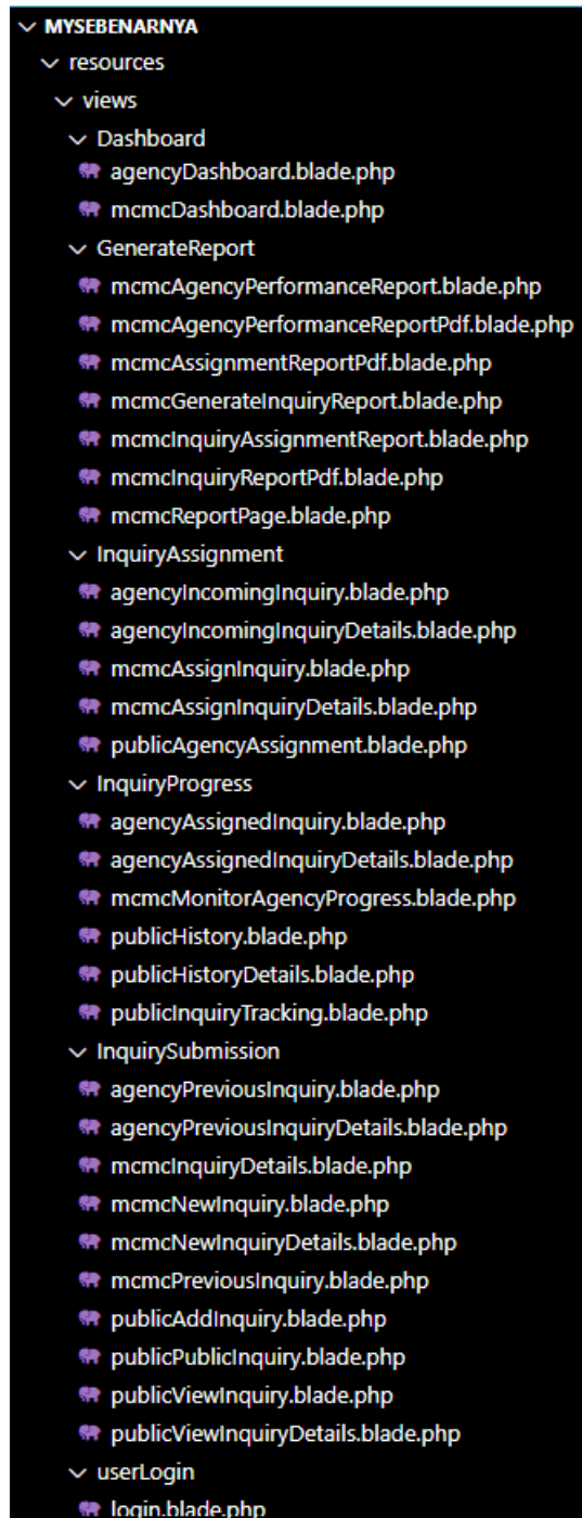
Figure 5. 1 Packages and its Classes in views
