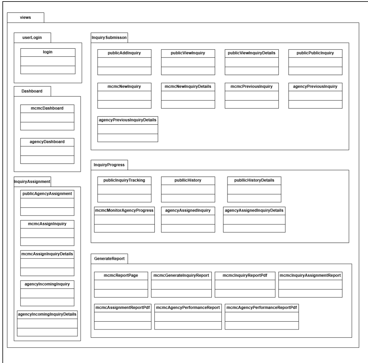
Figure 3. 1 Application Layer for MySebenarnya Systems
