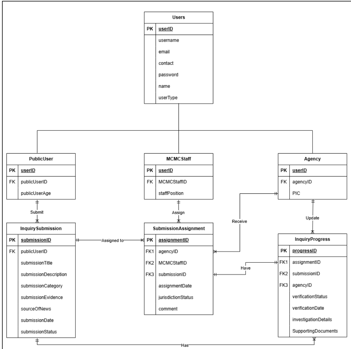
Figure 2. 1 Entity Relationship Diagram (ERD) for MySebenarnya System
