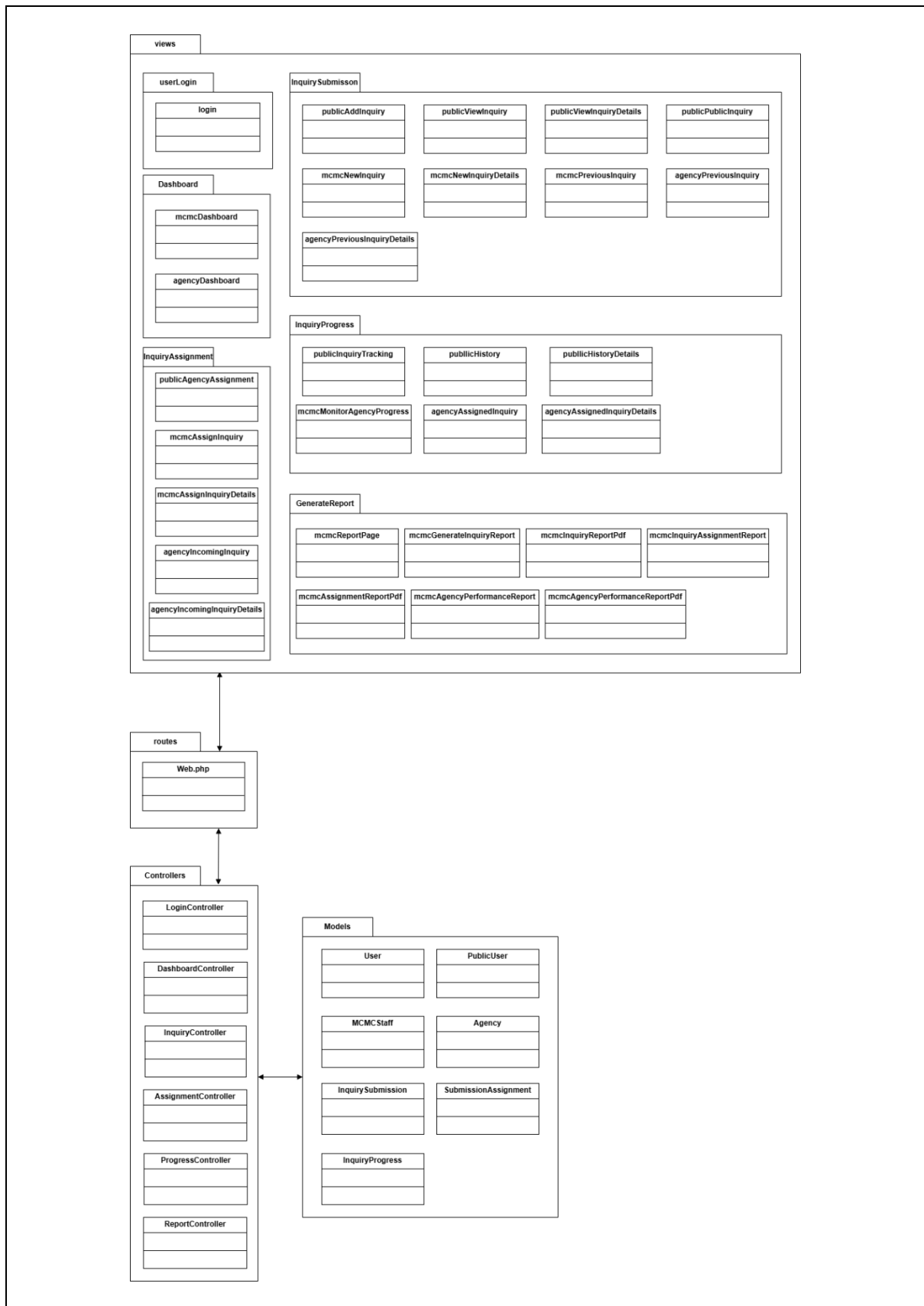
Figure 3. 4 Model View Controller (MVC) Package Relationship for MySebenarnya Systems
