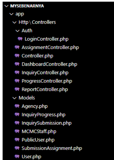
Figure 5. 2 Controller and Model
