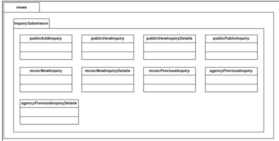
Figure 4. 1 Views for InquirySubmission Package
